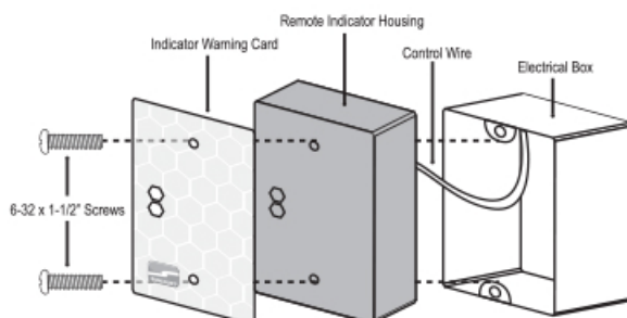
Figure 5: Mounting to Electrical Box
