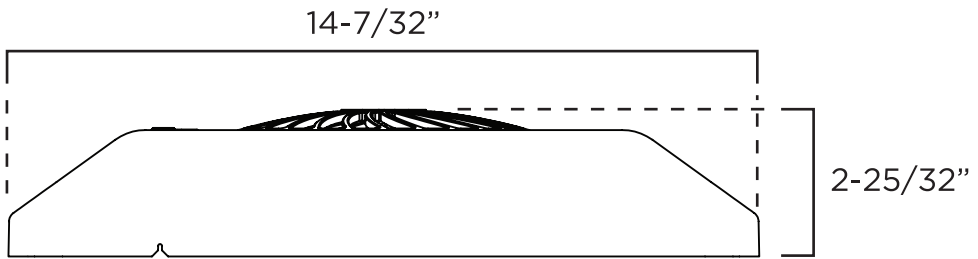
FRONT VIEW
