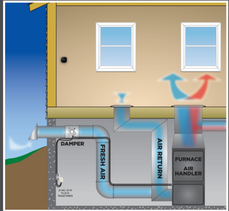
FRESH AIR INTAKE
