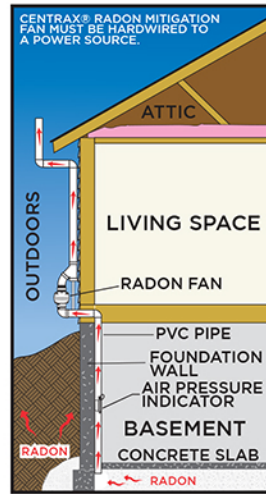
EXTERIOR INSTALLATION
