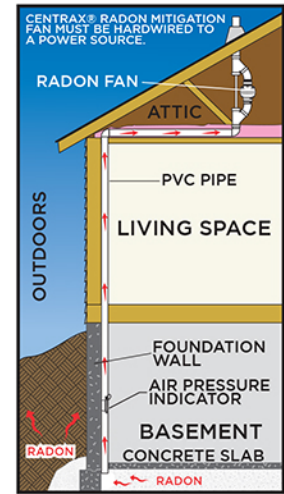
ATTIC INSTALLATION
