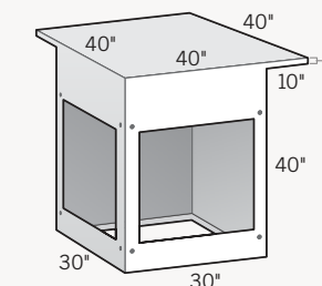
Bar-Height 90° Corner Cabinet with 10" Cantilever on Two Sides 30"D × 30"L × 40"H
