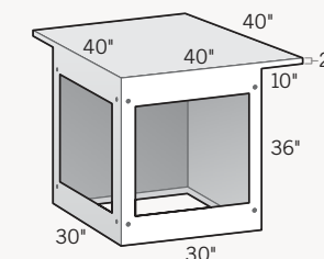
90° Corner Cabinet with 10" Cantilever on Two Sides 30"D × 30"L × 36"H
