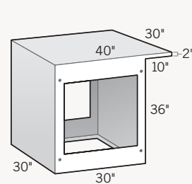
Cabinet with 10" Cantilever Backside 30"D × 30"L × 36"H
