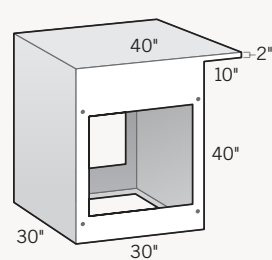
Bar-Height Cabinet with 10" Cantilever Backside 30"D × 30"L × 40"H
