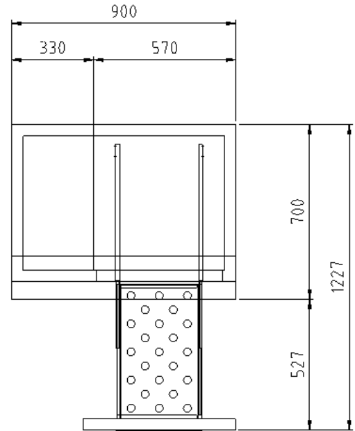
PLAN VIEW
