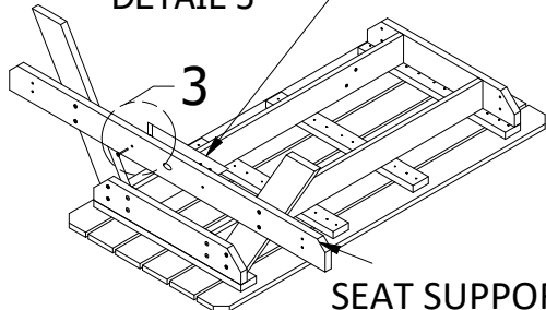
DETAIL 3
