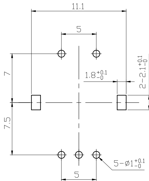
P.C.B.MOUNTING DETAIL
