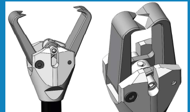
Jaw Type 1
