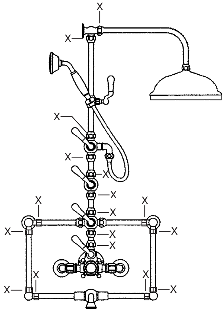
3/4" THERMOSTATIC VALVE
