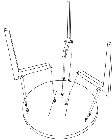
Bolts 9 Pieces
