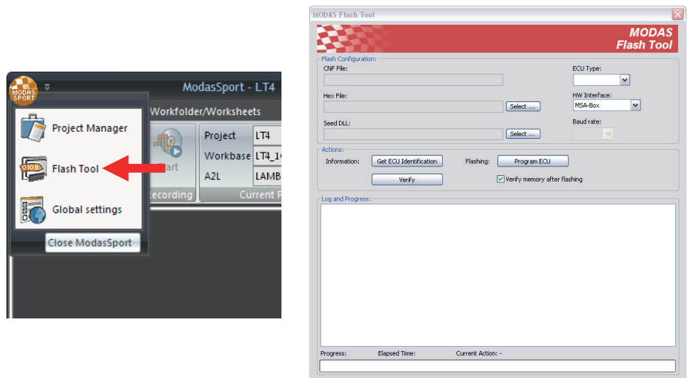
Fig. 5: Flash Tool selection and Modas Flash Tool window
