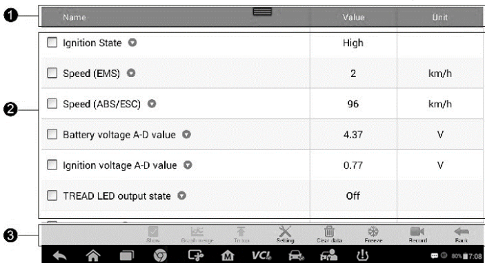
Figure 9-3 Sample Data Playback Screen
