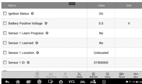
Figure 5-14 Sample Live Data Screen
