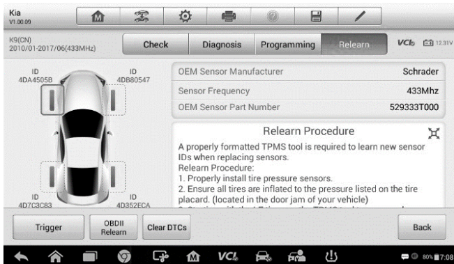
Figure 5-28 Sample OBD II Relearn Screen 1
