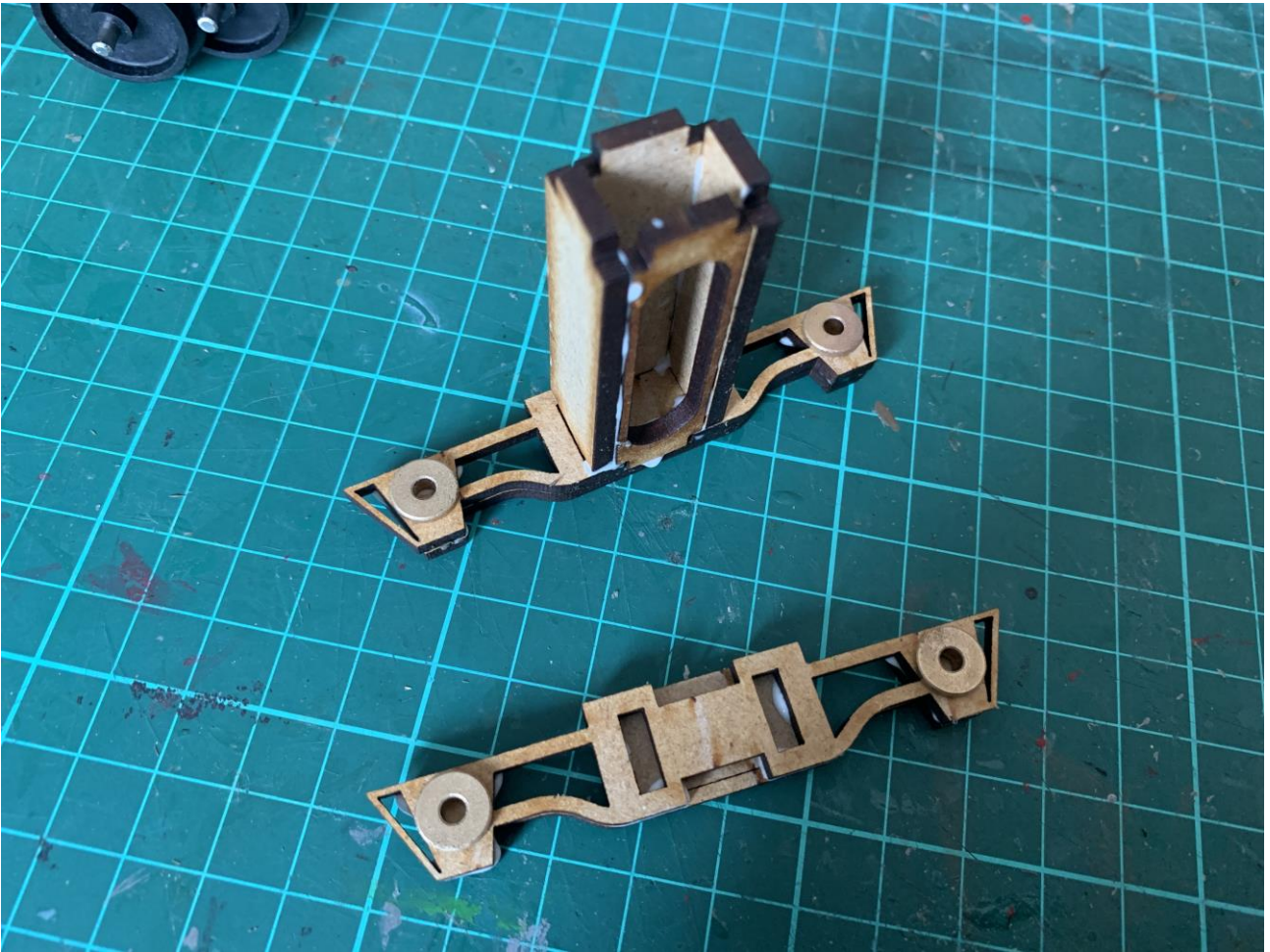
Start assembling the main bogie by gluing the centre cross beams onto one of the sides.
