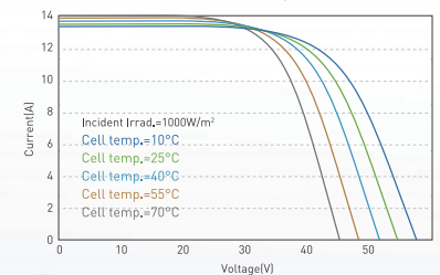
I-V Curve at Different Temperature (560W)
