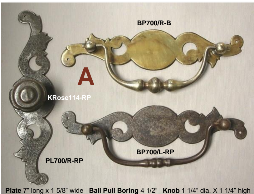
Plate 7" long x 1 5/8" wide Bail Pull Boring 4 1/2" Knob 1 1/4" dia. X 1 1/4" high
