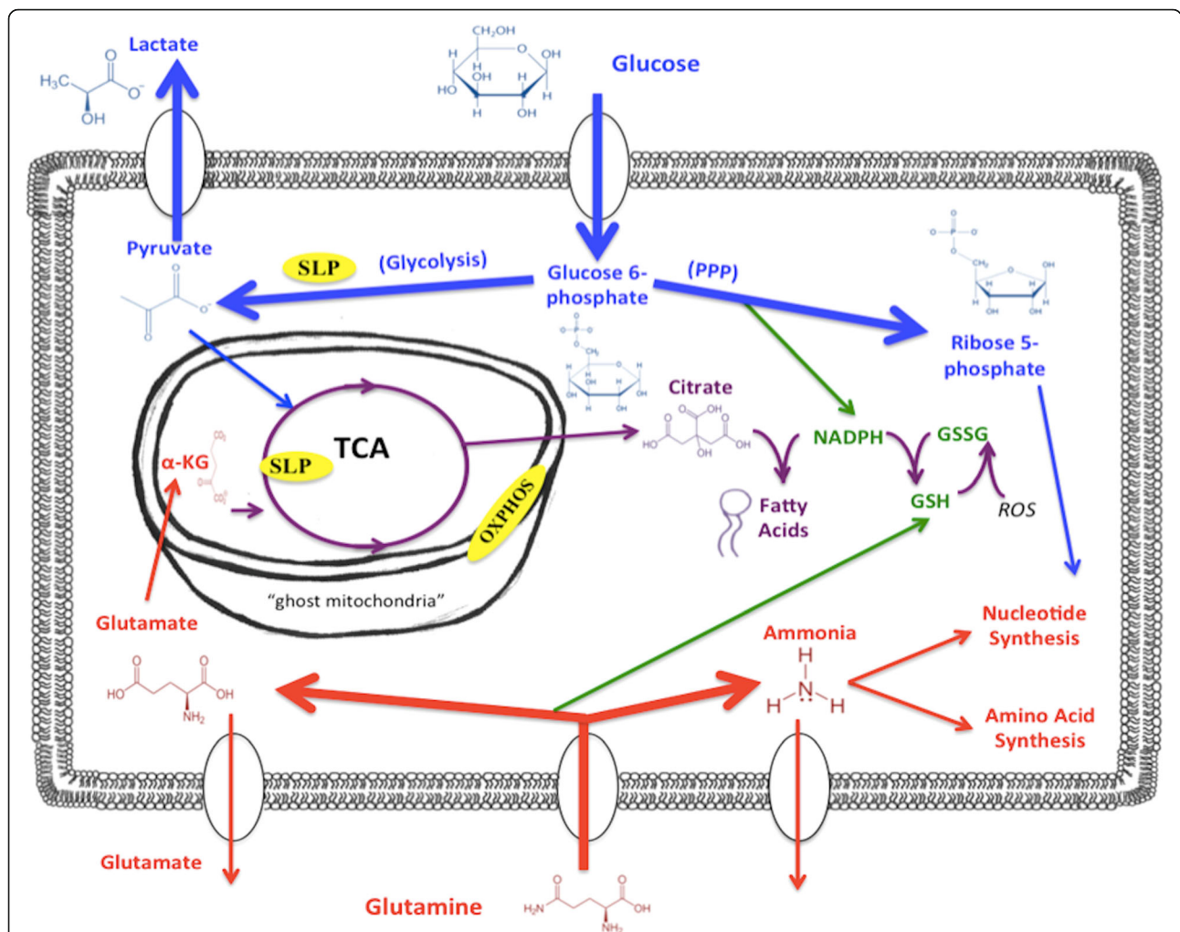
Fig. 1 Targeting Glucose and Glutamine for the Metabolic Management of Cancer. Cancer cells are largely dependent on glucose and glutamine for survival and growth. Energy through fermentation metabolism (substrate level phosphorylations, SLP) in glycolysis and the tricarboxylic acid cycle (TCA) will compensate for reduced energy through oxidative phosphorylation (OxPhos) that occurs in tumor cells. The yellow ovals indicate the three source of cellular ATP production. Glucose carbons can be used for both the glycolytic and pentose phosphate (PPP) pathways to supply ATP and precursors for lipid and nucleotide synthesis, as well as for glutathione production. Glutamine provides its amide nitrogen for ammonia and nucleotide synthesis. The glutamine-derived glutamate provides anapleurotic carbons to the TCA cycle through \alpha -KG for protein synthesis while also providing ATP through TCA cycle SLP. TCA cycle substrate level phosphorylation through the succinate thiokinase reaction can generate significant cellular ATP under hypoxia especially in tumor cells with defective respiration [78]. The glutamine-derived glutamate is also used for glutathione production that protects tumor cells from oxidative stress. Glucose and glutamine targeting will thus make cancer cells vulnerable to oxidative stress therapies. The simultaneous targeting of glucose and glutamine through the press-pulse therapeutic strategy will starve tumor cells of energy production while blocking their ability to synthesize proteins, lipids, and nucleotides. Glucose and glutamine can also be generated internally through the lysosomal digestion of phagocytosed glycoconjugates and proteins (see text). An elevation of non-fermentable ketone bodies through, calorie restriction, ketogenic diets, or supplementation will provide normal cells with an alternative energy source to glucose while also protecting them from oxidative stress. Ghost mitochondria are those containing little or no inner mitochondrial membranes (cristae), which are essential for normal OxPhos function [67, 282, 283]
