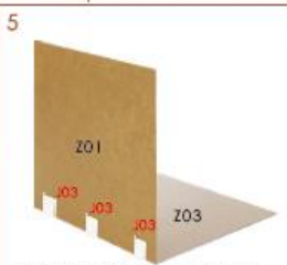
Use J03 to fix the junction of two pieces of plexiglass. (use transparent tape to replace J03)
