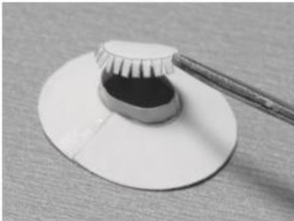
2. Assemble the A04-4-1,-2,-3 to finish the cap.
