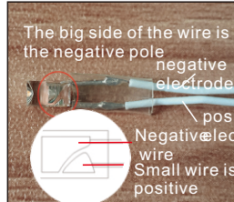
③ LED light positive and negative
