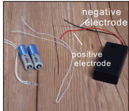
① Remove the battery box, LED lights, extension cords, tools: self-adhesive cloth, two batteries (battery-owned)
