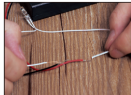
⑥ Connect the positive pole of the led lamp with the red line connecting the negative pole of the battery box and the black line (Connect the corresponding positive and negative poles)
