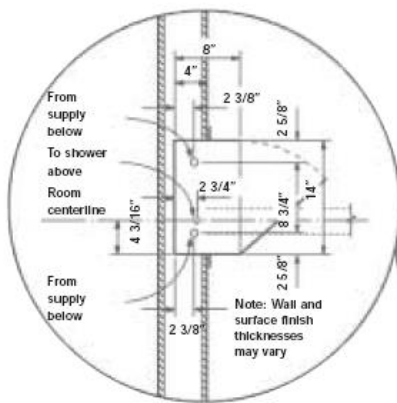
Plan Detail of Mixing Valve Pipe Rough-In
