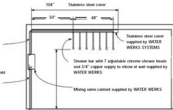
Typical Cross Section of Shower System
