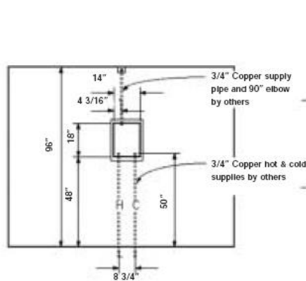
Mixing Valve Cabinet Rough-In Elevation
