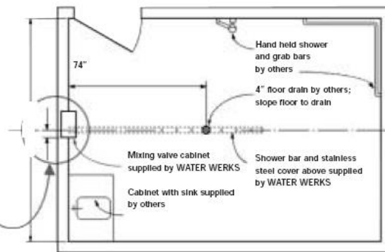
Typical Torrent Vichy Shower Room Plan
