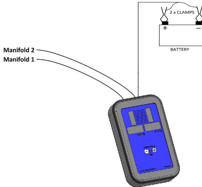
Figure 2 - Connection Diagram
