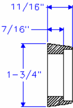
MODEL CGM
