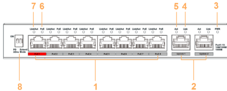
Figure 2-1 Front panel
