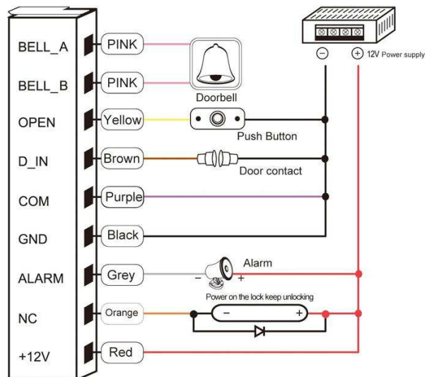
Common power supply diagram
