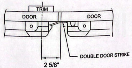
C. DOUBLE DOOR WITHOUT MULLION
