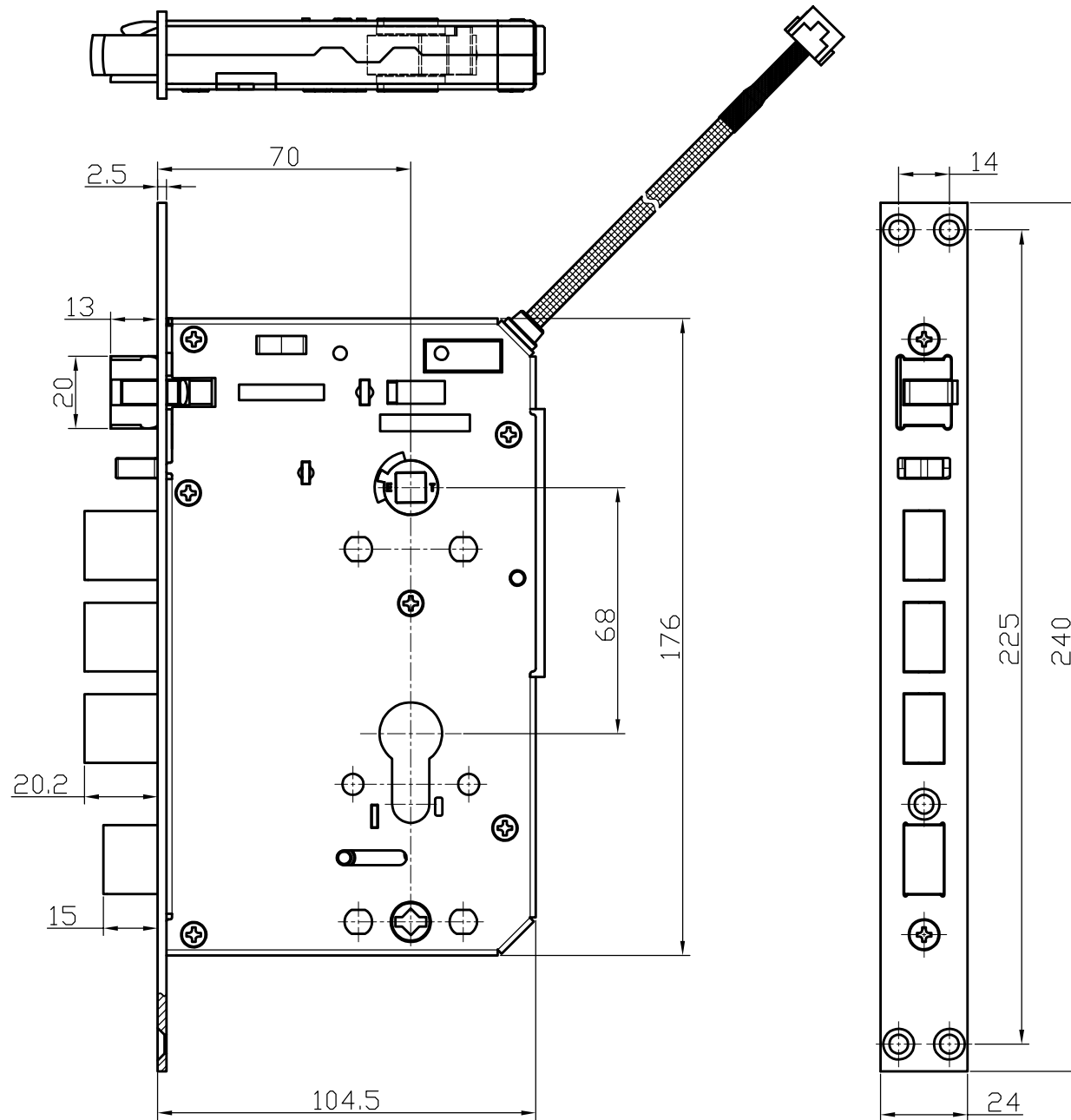
LOCKLY SECURE LUX (PGD829) MORTISE LOCK CASE
