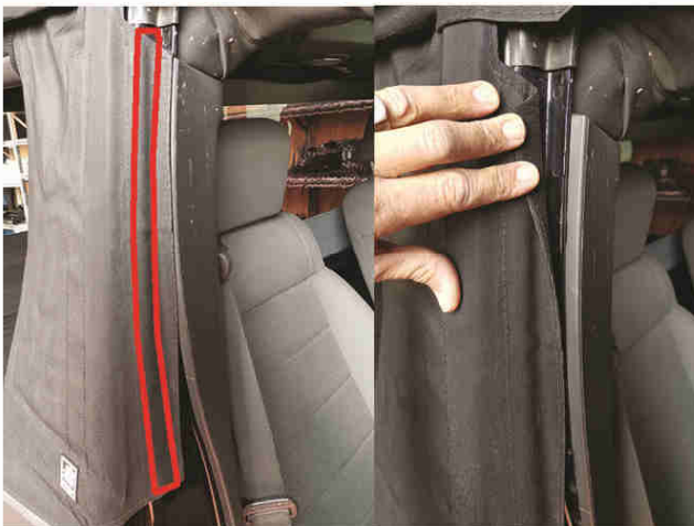
10 stick velcro on vertical struts of front door ( clean it before )
