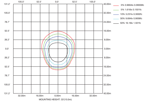
ISOLUX DIAGRAM
