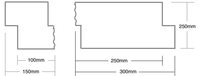
Corner Panel
