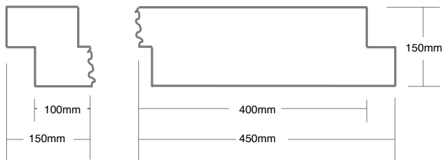
Corner Panel
