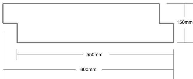
'Z' Panel
