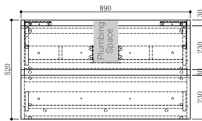
MIA 90W Front Section
