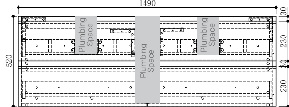
MIA 150SDW Front Section
