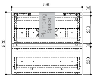
MIA 60W Front Section
