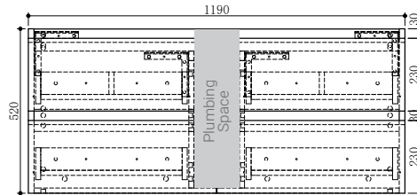
MIA 120SW Front Section
