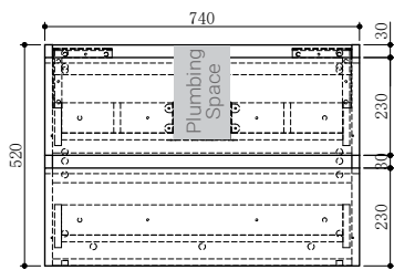
MIA 75W Front Section
