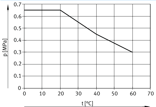
Operating pressure p as a function of temperature t (medium: water)
