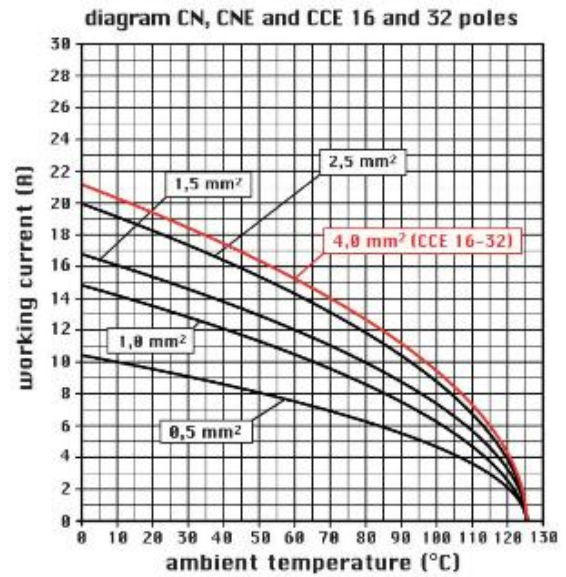
Catalogue drawings
