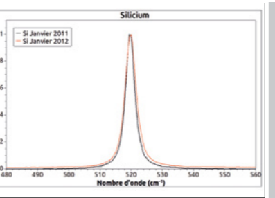
Si Raman Spectrum obtained with LSX-785S
