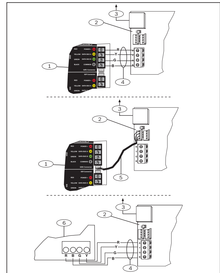
Figure 3.2: Wiring to the control panel (GV4 Series and FPD-7024 control panel shown)
