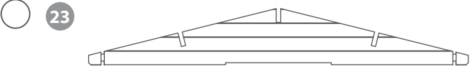
Gable Window Notch - 2996mm QTY 1 AI-0634RANE0403HGDD2SW-GW-V1
