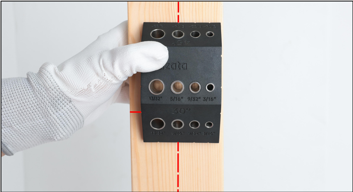
Step 2 - Align with the scales for accurate drilling.
