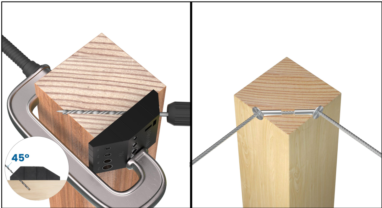
(45° for drilling corner post)
