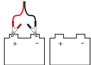
How NOT to wire alligator clips for 2 batteries
