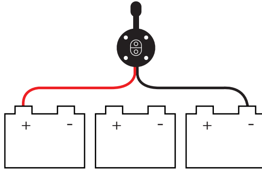
How TO wire a solar port for 3 batteries
