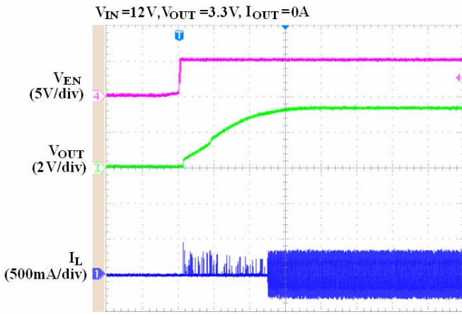
Times (4ms/div)
