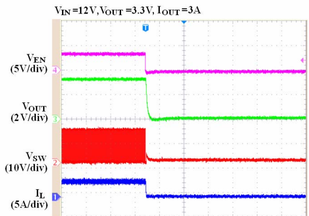
Times (200us/div)
