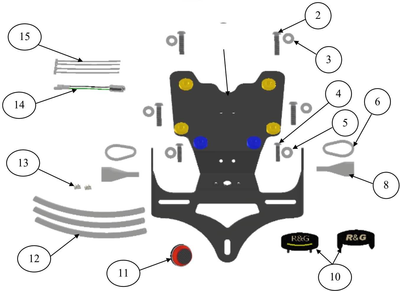
ASSEMBLY DIAGRAM
