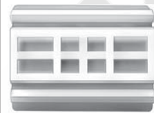
20782 (75306-SDA-A01) White Nylon Moulding Clip Head Size: 21mm x 27mm Stem Length: 11mm Accord 2003 - On UNIT PACKAGE: 10
