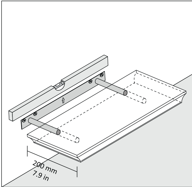
PROFILE 200 mm | 8 in
