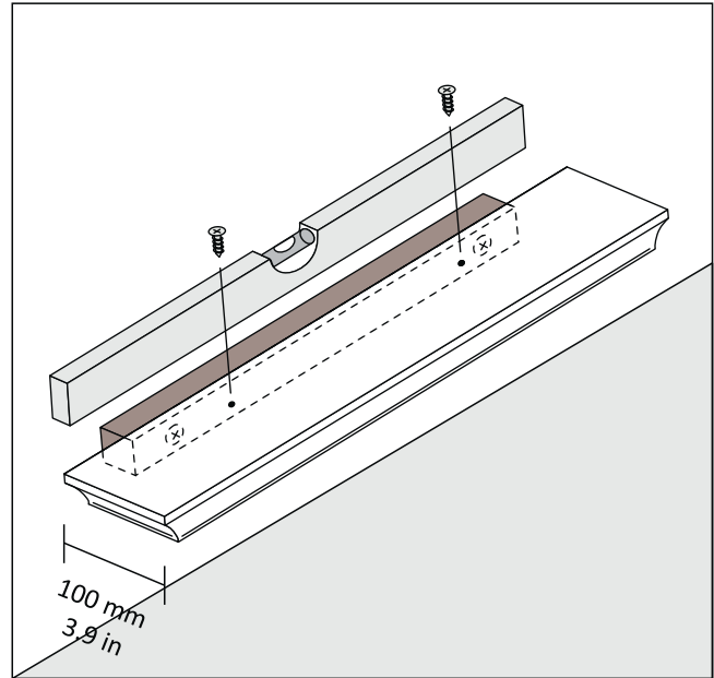
PROFILE 100 mm | 4 in
