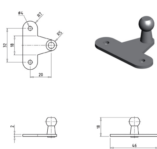
PART NO: BRACKET-08
