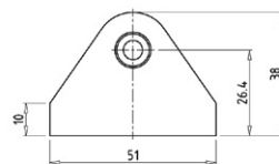
PART NO: BRACKET-04
