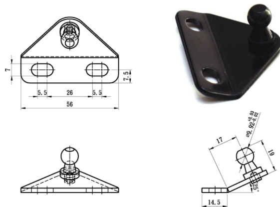
PART NO: BRACKET-52
