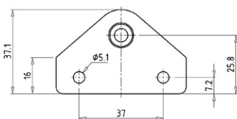
PART NO: BRACKET-05
