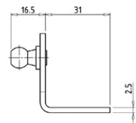
PART NO: BRACKET-04
