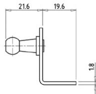
PART NO: BRACKET-03
