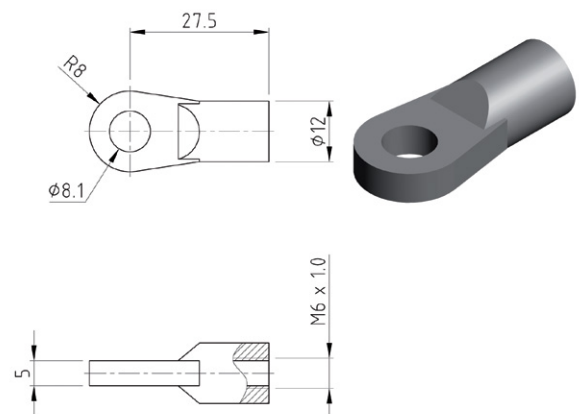
PART NO: D8A-2 STAINLESS STEEL PART NO : A15S08M- 6SUS303
