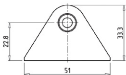
PART NO: BRACKET-03
