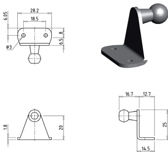
PART NO: BRACKET-07
