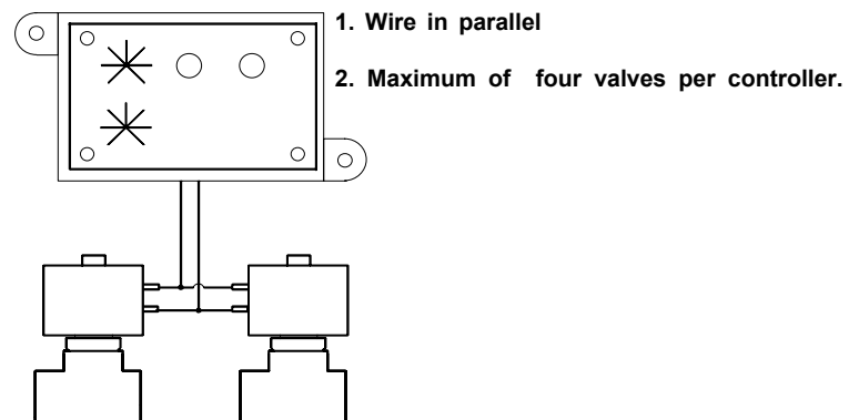
DIAGRAM 2 - WIRING MULTI-VALVE DRAIN
