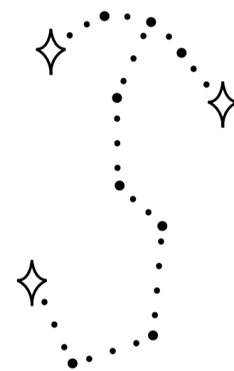
Scorpio Constellation
