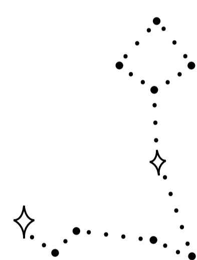
Pisces Constellation
