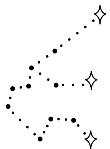
Aquarius Constellation
