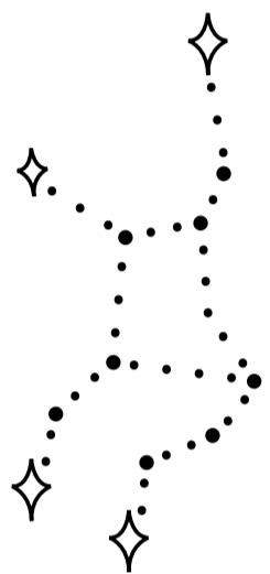
Virgo Constellation
