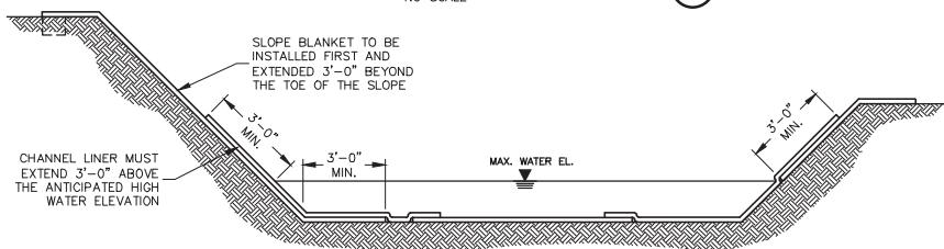
CHANNEL INSTALLATION METHOD "B" NO SCALE (3/10)
