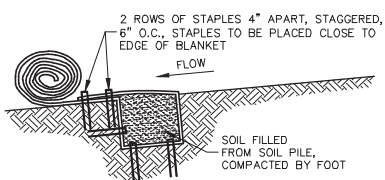
CHANNEL TRENCHING METHOD "B" NO SCALE (9/10)
