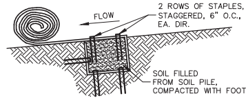
CHANNEL TRENCHING METHOD "A" NO SCALE (8/10)
