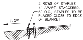
CHANNEL TERMINATION NO SCALE (5/10)
