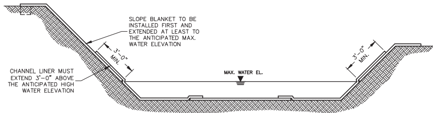
CHANNEL INSTALLATION METHOD "A" NO SCALE (2/10)
