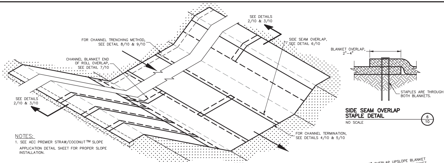
CHANNEL DETAIL NO SCALE (1/10)
