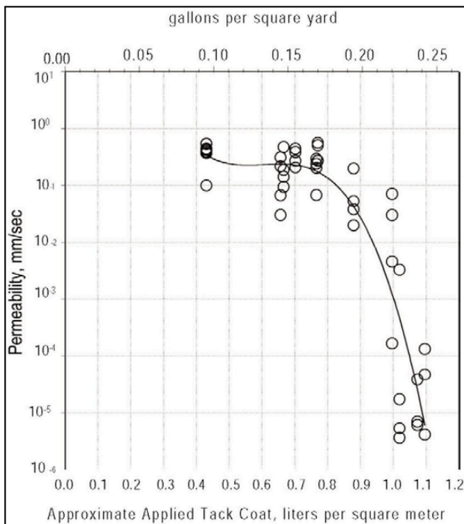
Figure 1 - Paving Fabric Permeability as a Function of Tack Coat Application
