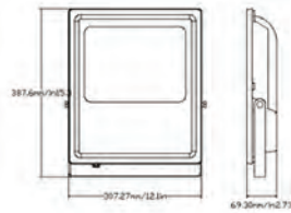
FLOOD-150W 150W
