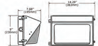
WALL-PACK 60W
