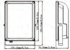
FLOOD-50 50W
