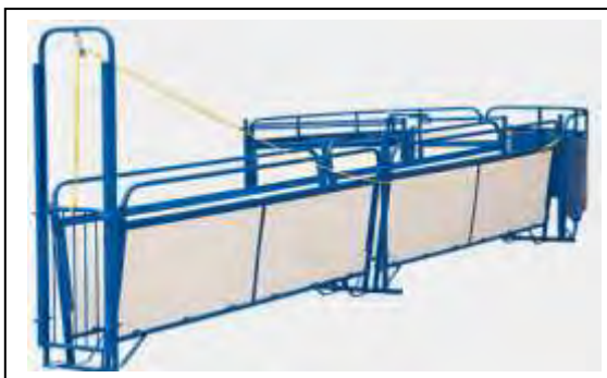
WCCT WORKING CHUTE/CROWDING TUB Quick, safe way to handle your sheep. All sections of chute can be interchanged Length of chute can be extended Guillotines and anti-backups can be inserted anywhere along chute
