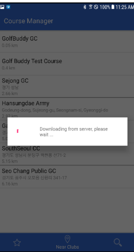
> Update Process
